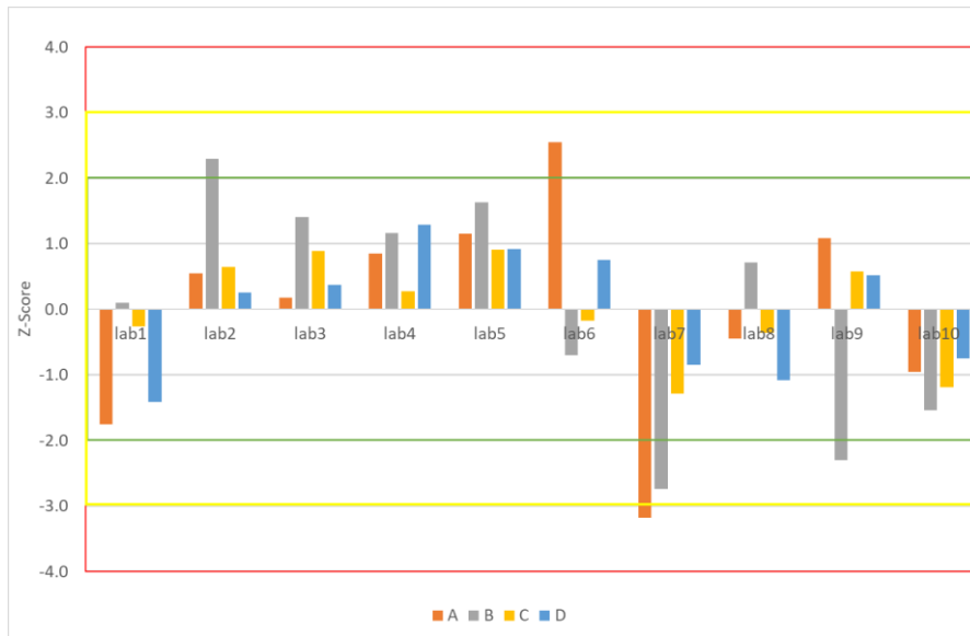
Figure 5 Z-Score of the results for a onefold SD of 0.5°C
