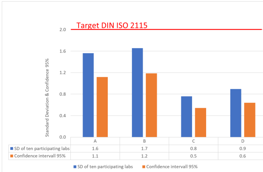
Figure 3 Standard Deviation and confidence level of the MFFT results between the company labs
